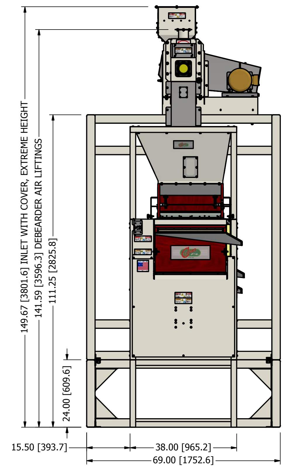
FRONT VIEW; DEBEARDER MINI, ECLIPSE 324, DEBEARDER SURGE HOPPER, ECLIPSE 324 5 BUSHEL SURGE HOPPER, FAN AIR TRANSITION & 24" STAND FACTORY
