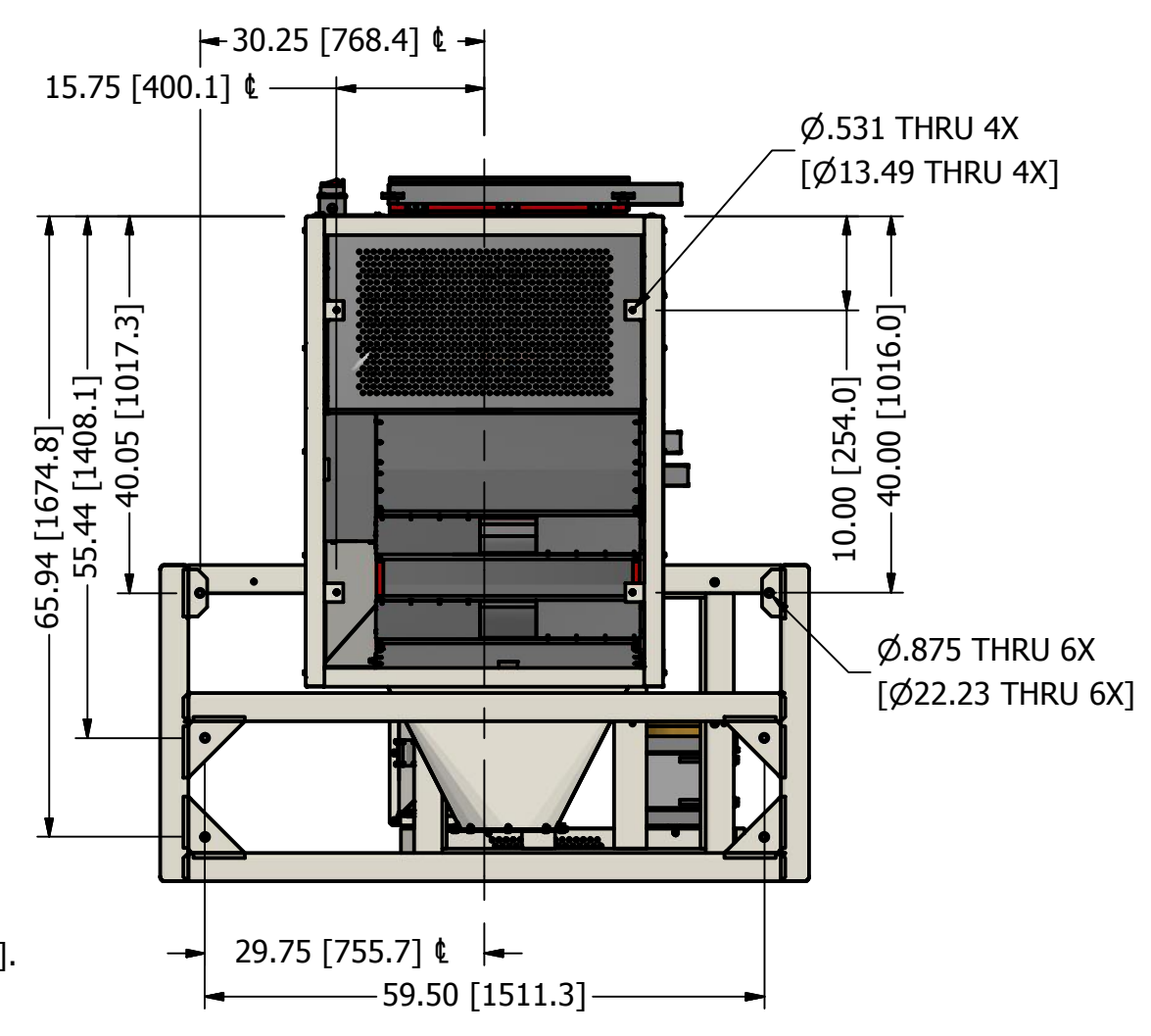
FRONT VIEW; DEBEARDER MINI, ECLIPSE 324, DEBEARDER SURGE HOPPER, ECLIPSE 324 5 BUSHEL SURGE HOPPER, FAN AIR TRANSITION & 24" STAND FACTORY
