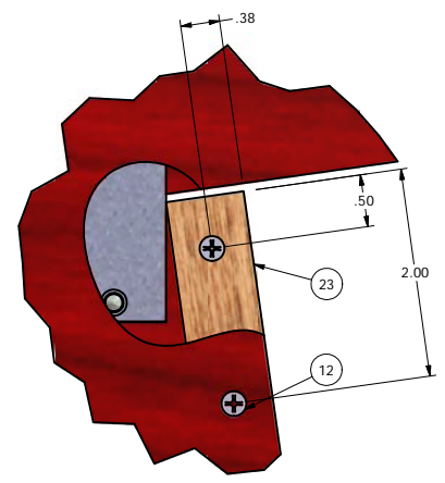
DETAIL H SCALE 1
