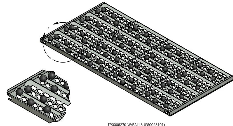
DETAIL F SCALE 3/16 5 BALLS (F80026102) PER COMPARTMENT 80 BALLS PER TRY
