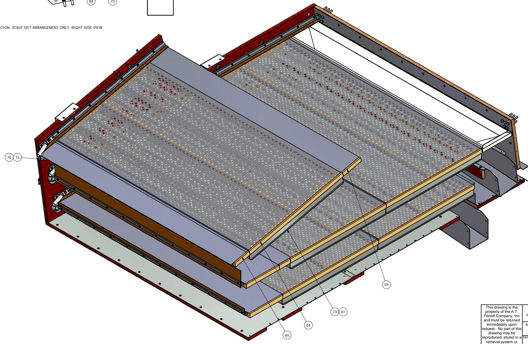
SCREEN INSTALLATION, SCALP SIFT ARRANGEMENT ONLY
