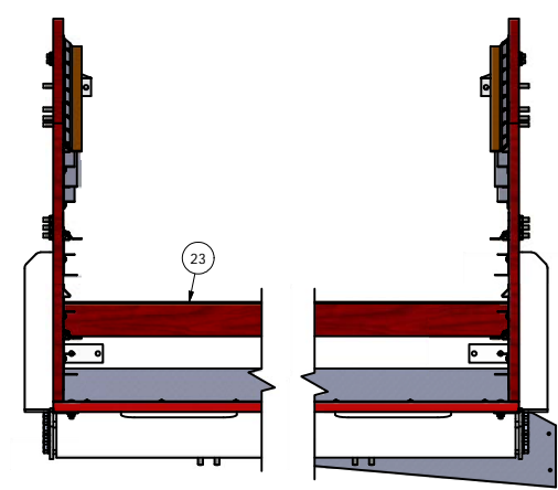
STEP #8: INNER CROSSBOARD INSTALLATION, FRONT VIEW SCALE 1/8
