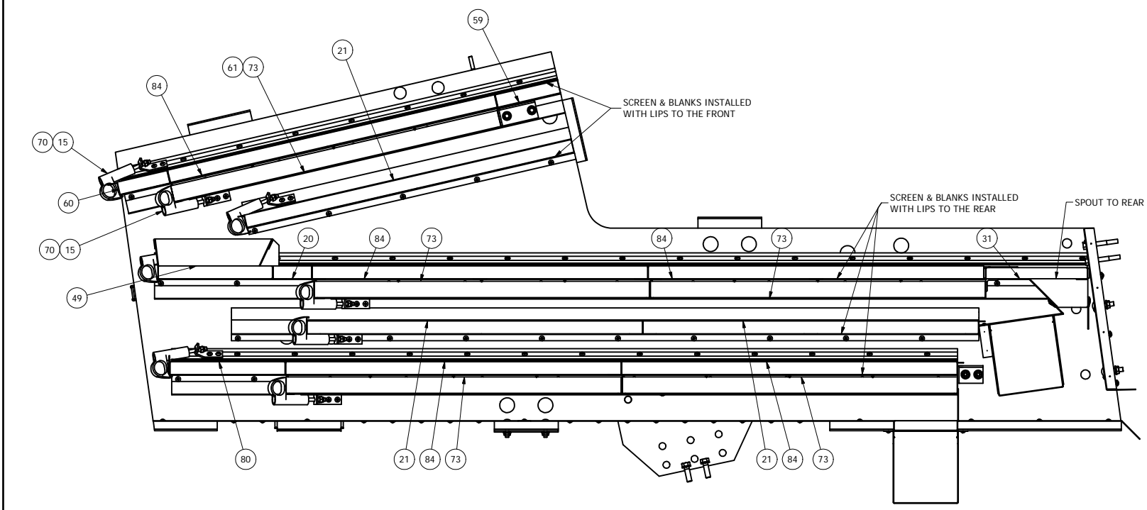
SCREEN INSTALLATION, SPLIT SIFT ARRANGEMENT ONLY, RIGHT SIDE VIEW
