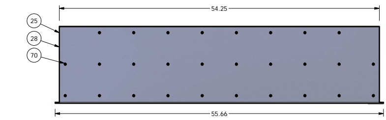
STEP #7: FRONT VIEW, BACK BOARD ASSY SCALE 1/8
