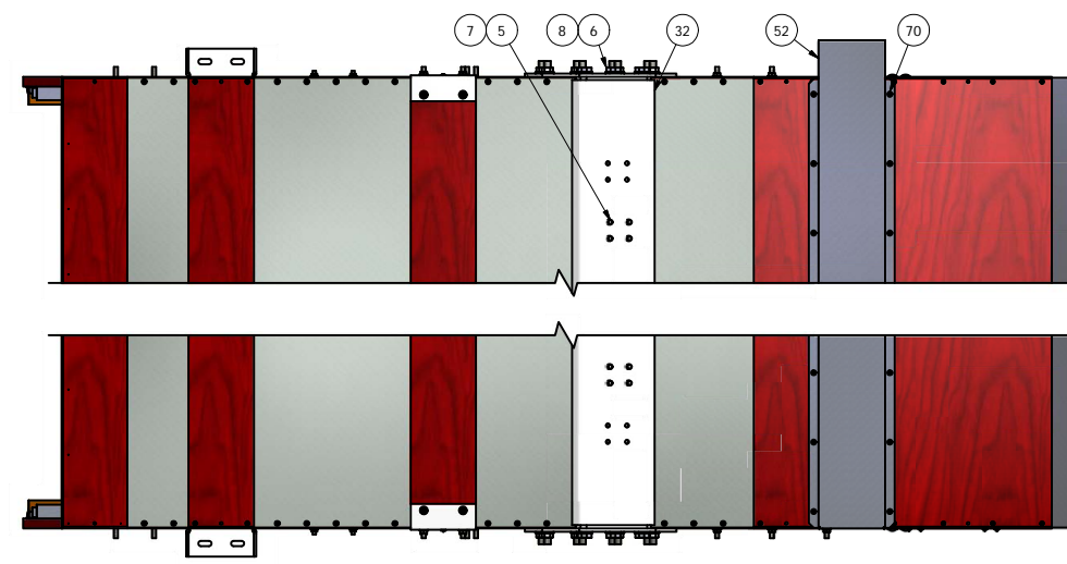
STEP #5: RIGHT SIDE VIEW, SPOUT BRIDGE FASTENER & PITMAN TUBE ASSY SCALE 1/8 RIGHT HAND ASSY SHOWN, INSTALL (F61001258) OPPOSITE FOR LEFT HAND.
