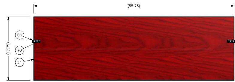
STEP #6: FRONT VIEW, DOOR ASSY SCALE 1/8
