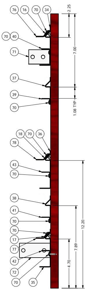
SECTION A-A SCALE 3/8
