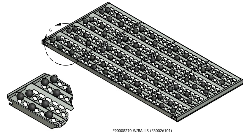
DETAIL G SCALE 3/16 5 BALLS (F80026102) PER COMPARTMENT 80 BALLS PER TRY
