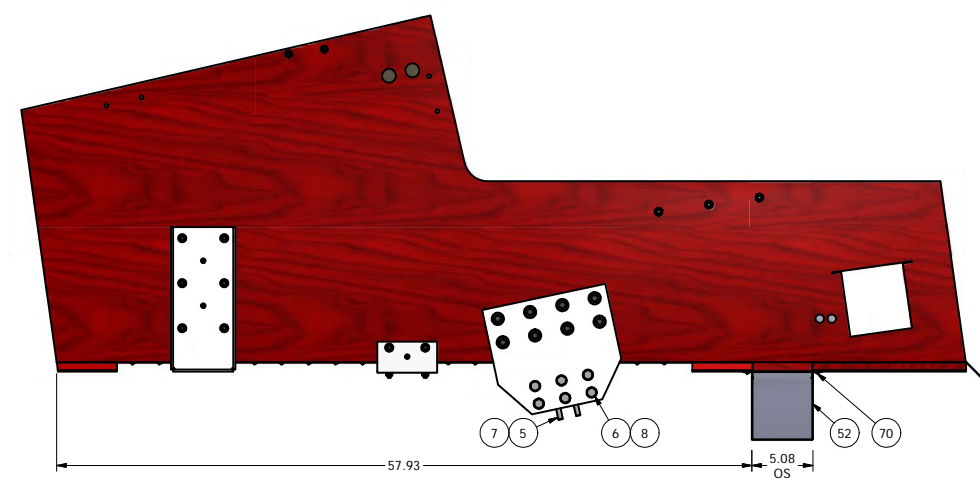
STEP #5: RIGHT SIDE VIEW, SPOUT BRIDGE FASTENER & PITMAN TUBE ASSY SCALE 1/8 RIGHT HAND ASSY SHOWN, INSTALL (F61001258) OPPOSITE FOR LEFT HAND.
