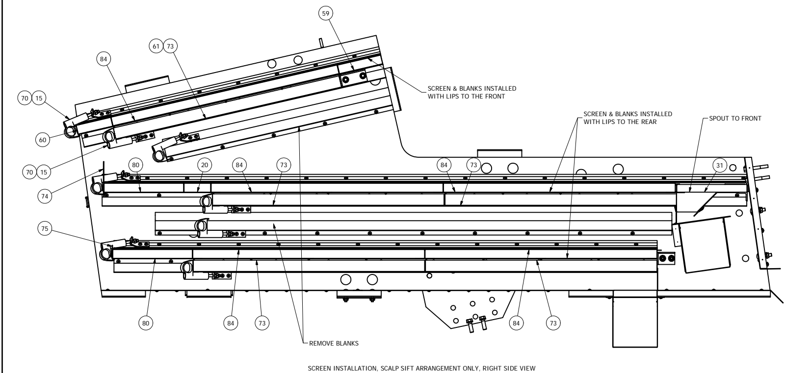
SCREEN INSTALLATION, SCALP SIFT ARRANGEMENT ONLY, RIGHT SIDE VIEW
