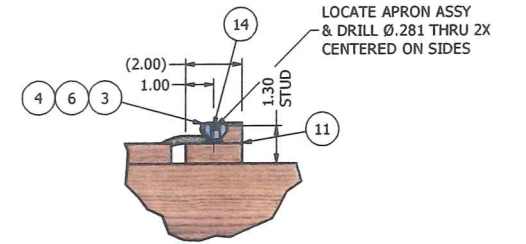
DETAIL E SCALE 0.31 : 1
