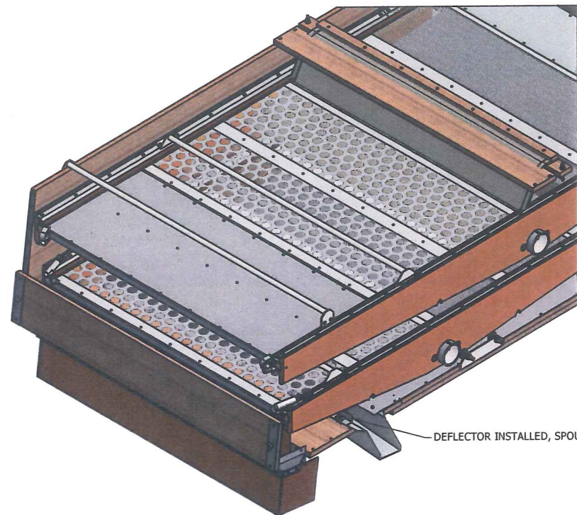
RIGHT SIDE CUTAWAY, DEFLECTOR INSTALLED SCALE 1/8
