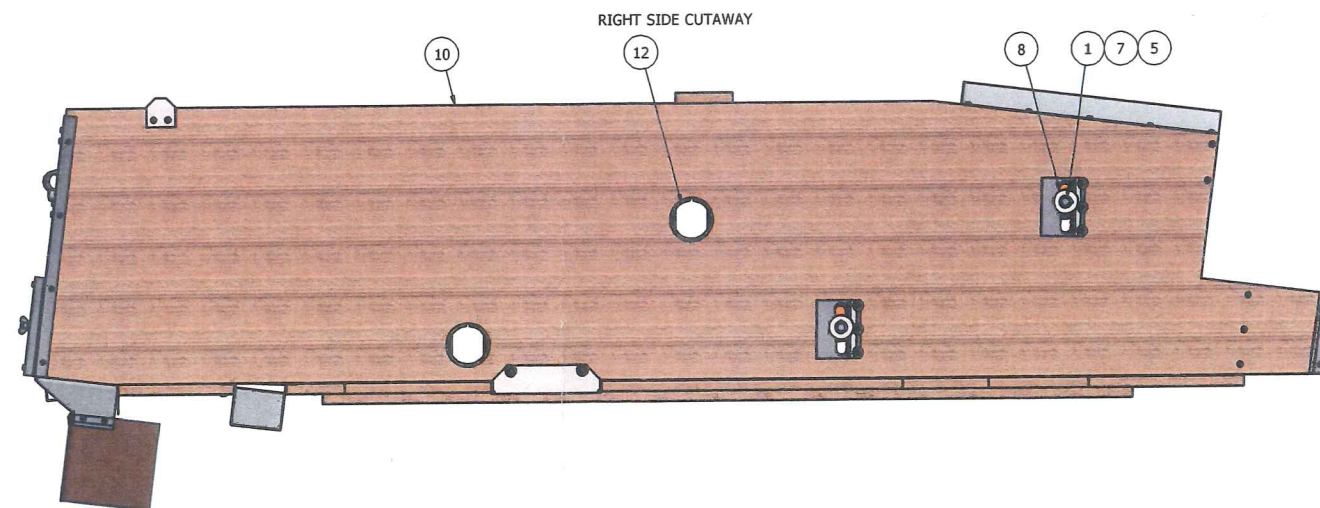
STEP 2: RIGHT SIDE VIEW, TOP ROCKER INSTALLATION
