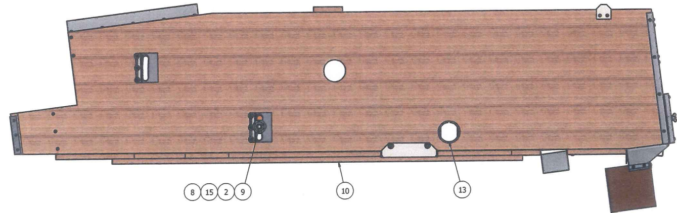
STEP 1: LEFT SIDE VIEW, BOTTOM ROCKER INSTALLATION
