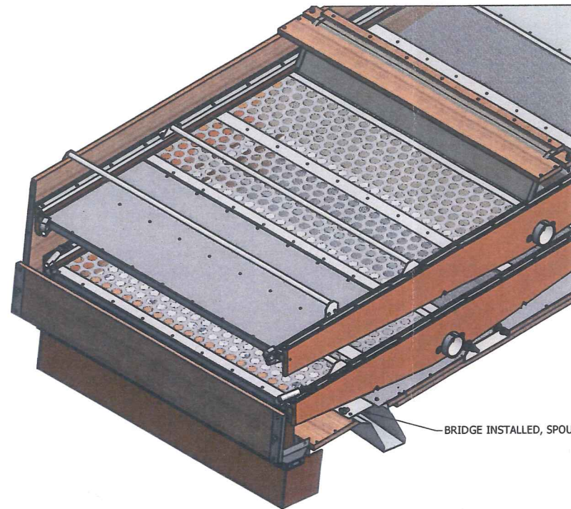
RIGHT SIDE CUTAWAY, BRIDGE INSTALLED SCALE 1/8
