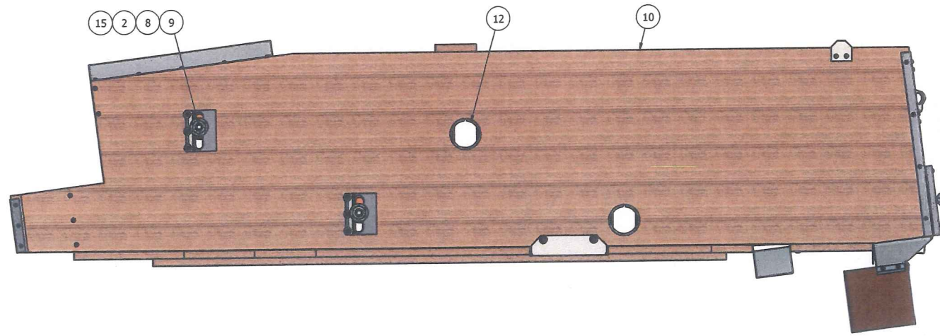
STEP 2: LEFT SIDE VIEW, TOP ROCKER INSTALLATION
