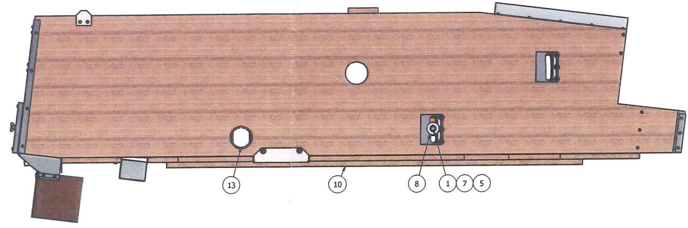
STEP 1: RIGHT SIDE VIEW, BOTTOM ROCKER INSTALLATION
