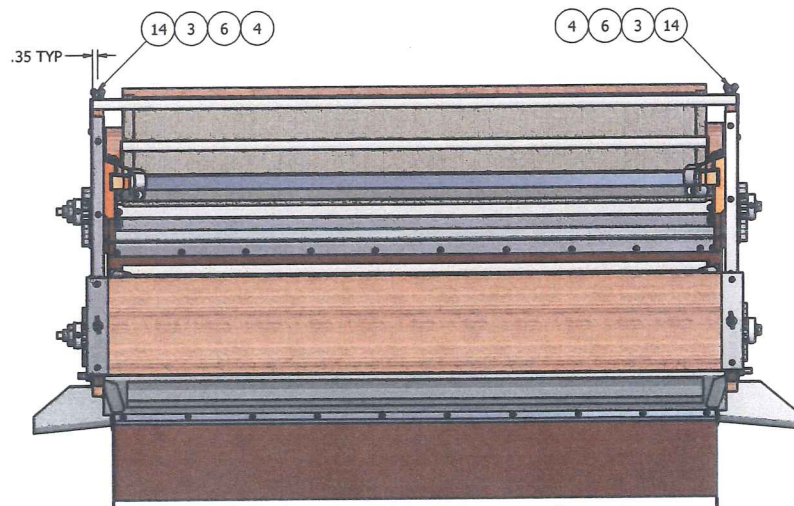
RIGHT SIDE CUTAWAY, DEFLECTOR INSTALLED SCALE 1/8
