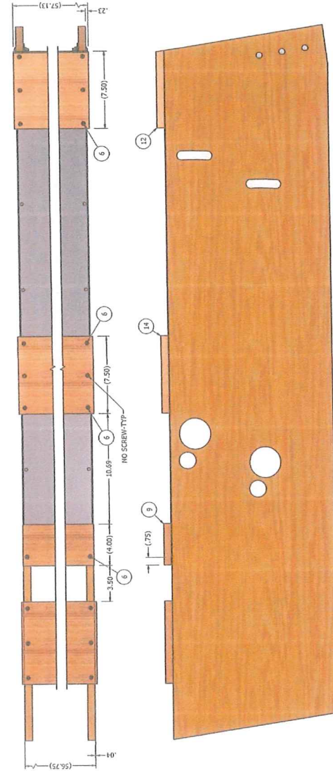
STEP 1: ISOMETRIC VIEW, UPSIDE DOWN BOTTOM CROSS BOARD INSTALLATION
