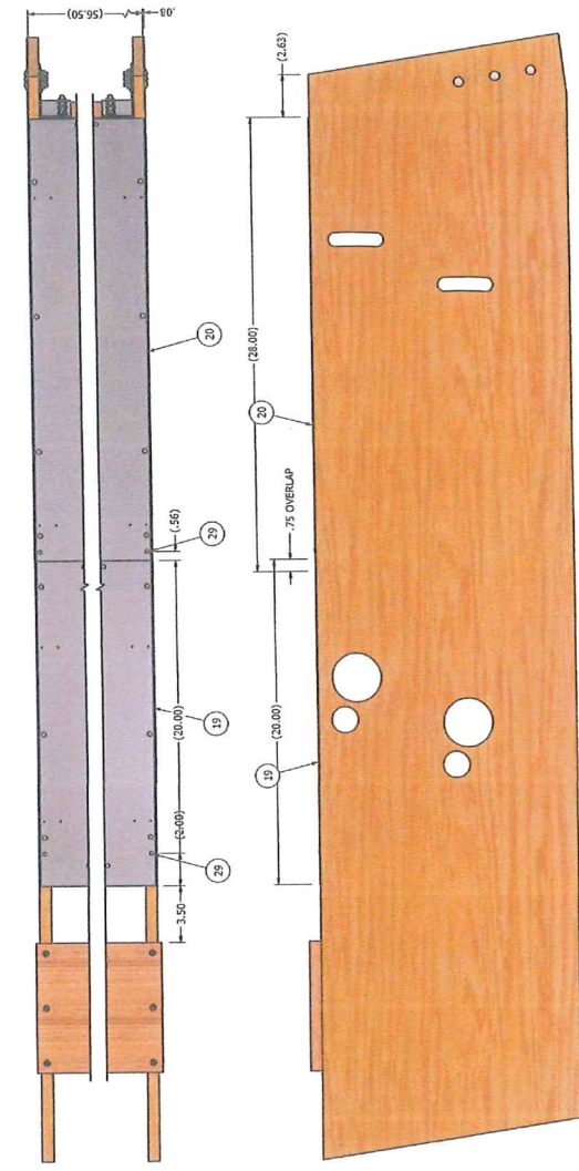
STEP 2: RIGHT SIDE VIEW, UPSIDE DOWN SHOE BOTTOM METAL INSTALLATION
